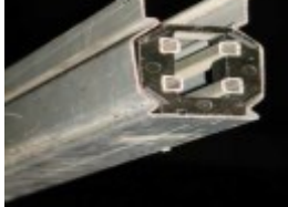
GE Flex-O-Power 50 Amps, 300 volt, 4 pole 10' rails, 220v & 110v
